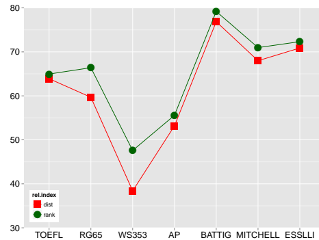
Figure 17: Reduced Setting
