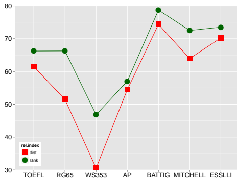
Figure 16: Unreduced Setting
