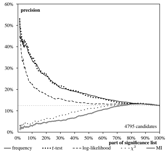
Figure 3: Newsgroup f \geq 5 : prec. curves 1
